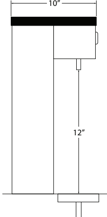
CM-2PB-RDP Side View
