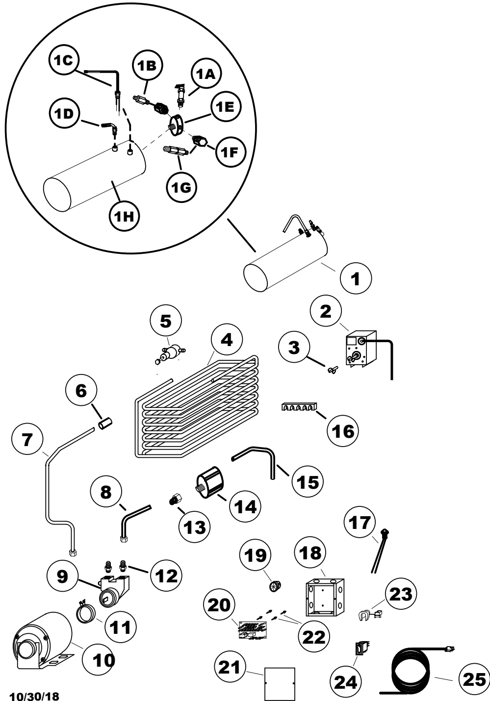
10/30/18 Drawing #12
